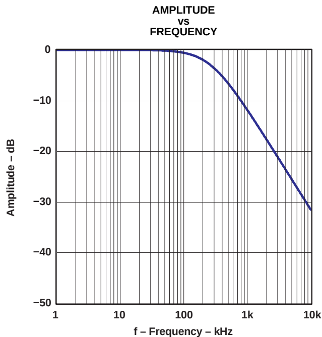
Figure 29. Stop-Band Characteristic
