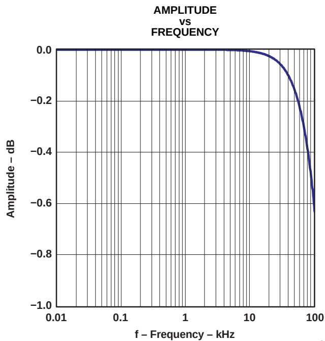
Figure 30. Pass-Band Characteristic
