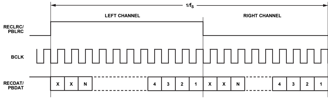
Figure 24. Right-Justified Audio Input Mode
