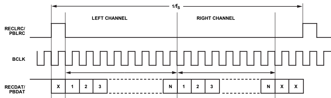
Figure 27. DSP/PCM Mode Audio Input Submode 2 (SM2) [Bit LRP = 1]
