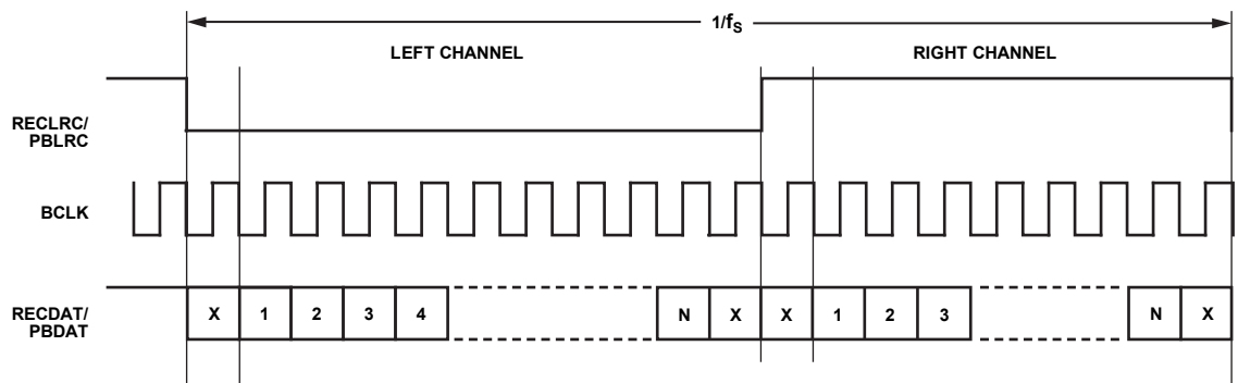
Figure 25. I S Audio Input Mode
