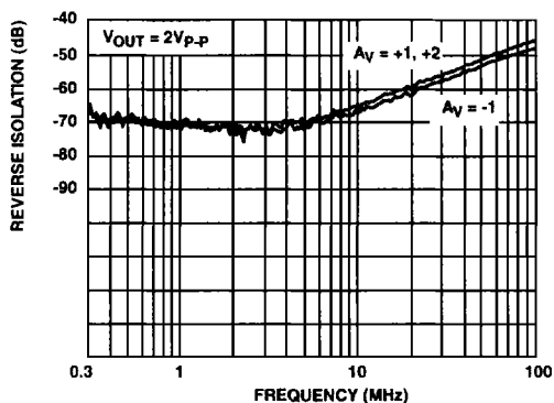
FIGURE 19. REVERSE ISOLATION
