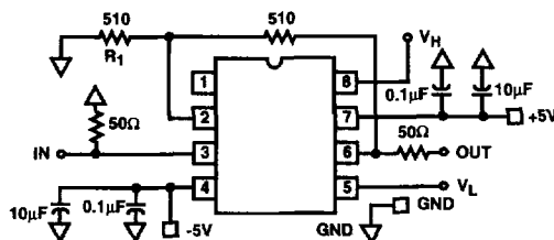
FIGURE 2C. SCHEMATIC
