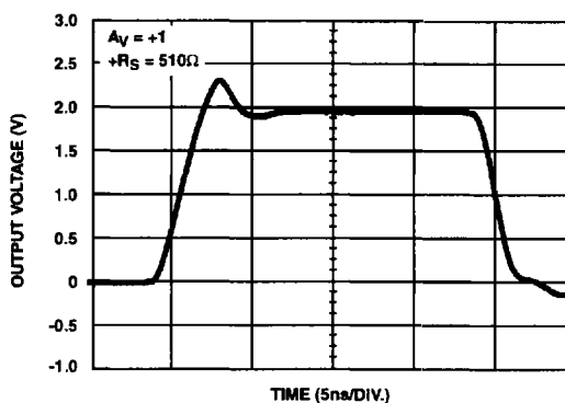
FIGURE 4. LARGE SIGNAL POSITIVE PULSE RESPONSE
