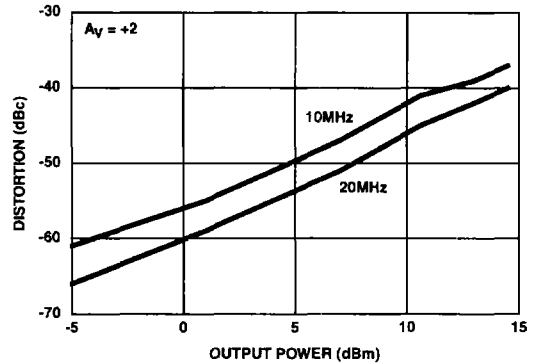
FIGURE 22. SECOND HARMONIC DISTORTION vs P_{\text{OUT}}
