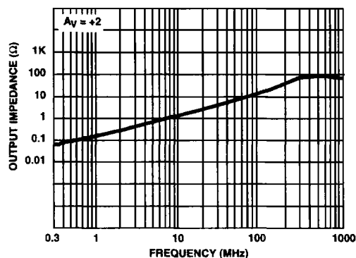
FIGURE 20. OUTPUT IMPEDANCE
