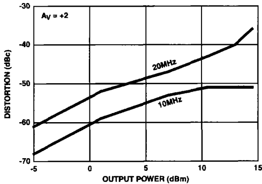
FIGURE 23. THIRD HARMONIC DISTORTION vs P_{\text{OUT}}
