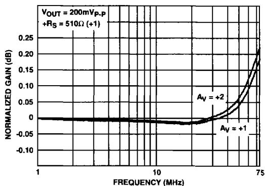
FIGURE 18. GAIN FLATNESS
