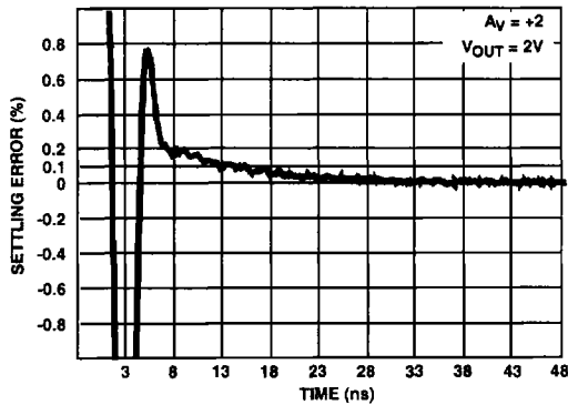
FIGURE 21. SETTLING RESPONSE
