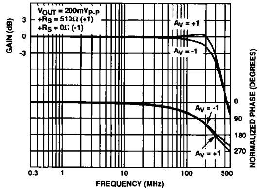
FIGURE 12. FREQUENCY RESPONSE
