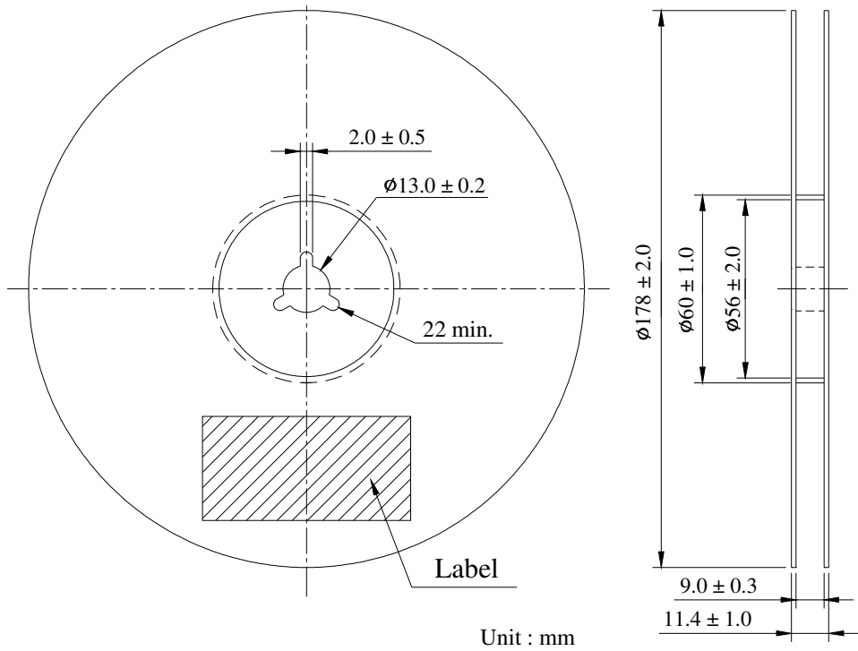
9-1-3 Reel dimensions( Material : Polystyrene )
